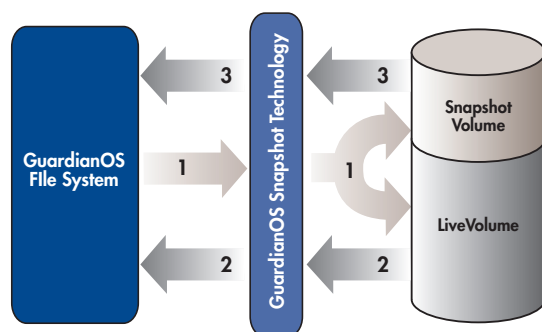
Figure 2. GuardianOS Snapshot Copy-on-Write Operation
