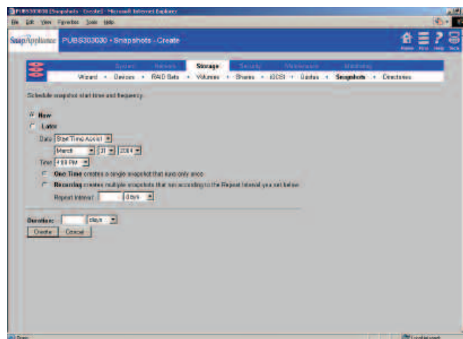
Figure 3. GuardianOS Snapshot Scheduling
